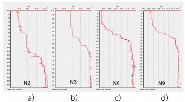
Figure 9 Halocline in the survey station of the North Coast of Timor-Leste, 2019 a) N2 b) N3 c) N4 d) N9
