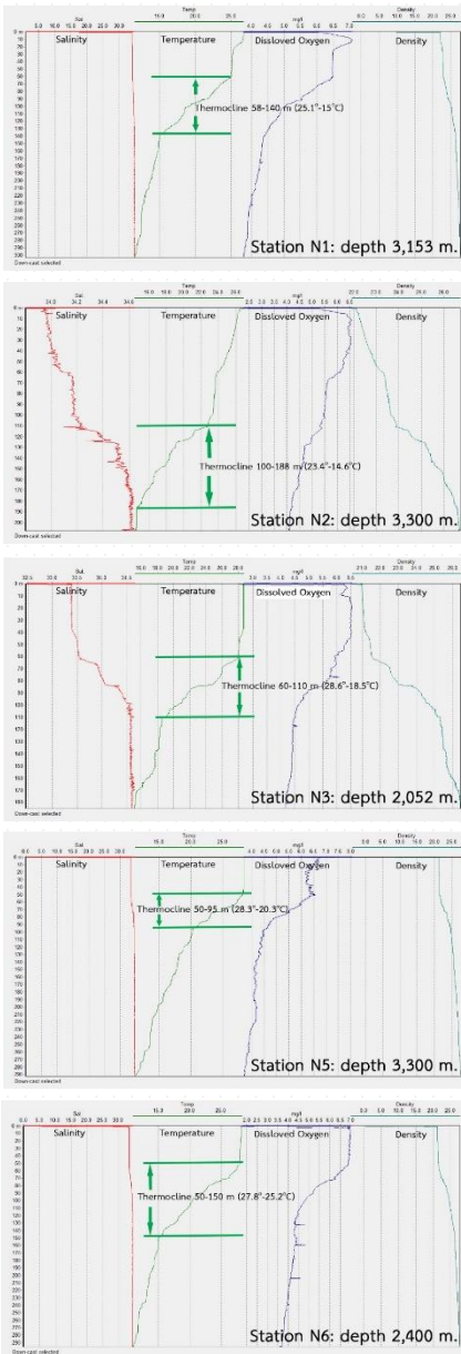
Figure 8 Thermocline, salinity and dissolved oxygen in the survey stations of the North Coast of Timor-Leste, 2019 a) N1 b) N2 c) N3 d) N5 e) N6
