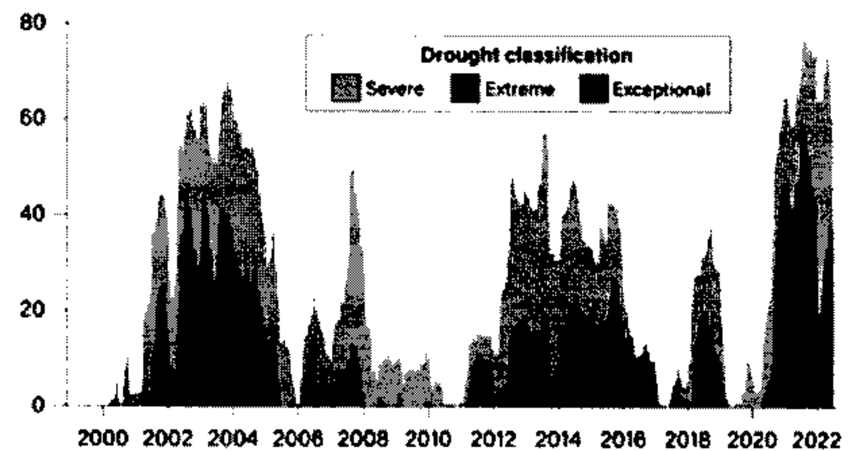
Percent of western land area experiencing drought
